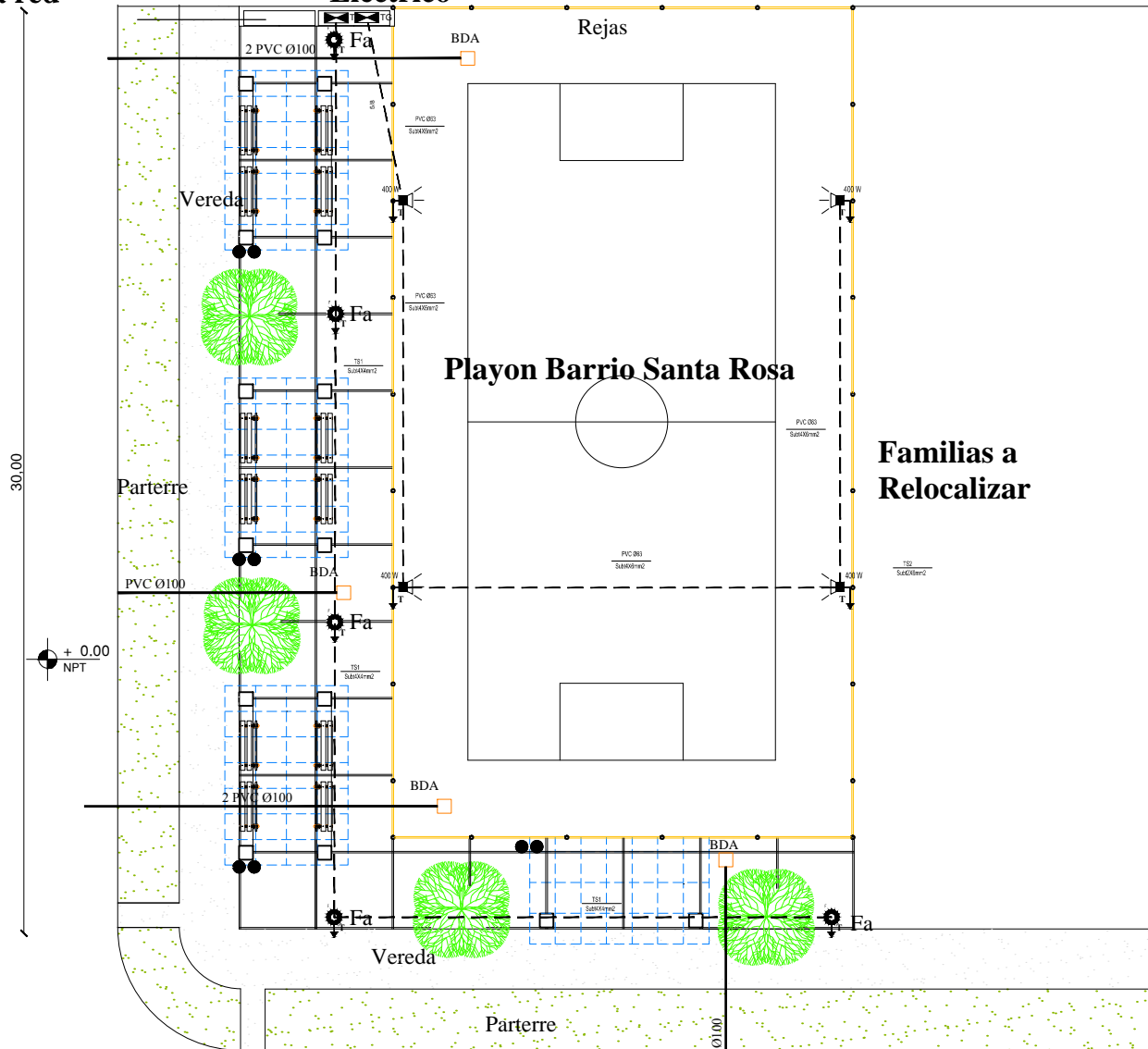
PLANTA PLAYON SANTA ROSA
